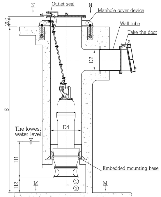
2. Precast concrete shaft installation
